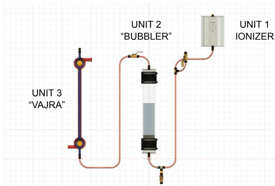
The Thunderstorm Generator – Overview of the complete system – Credit Nykyta Vovk
