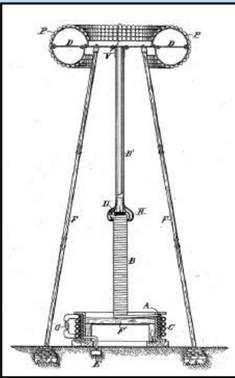
Tower Cross Section
